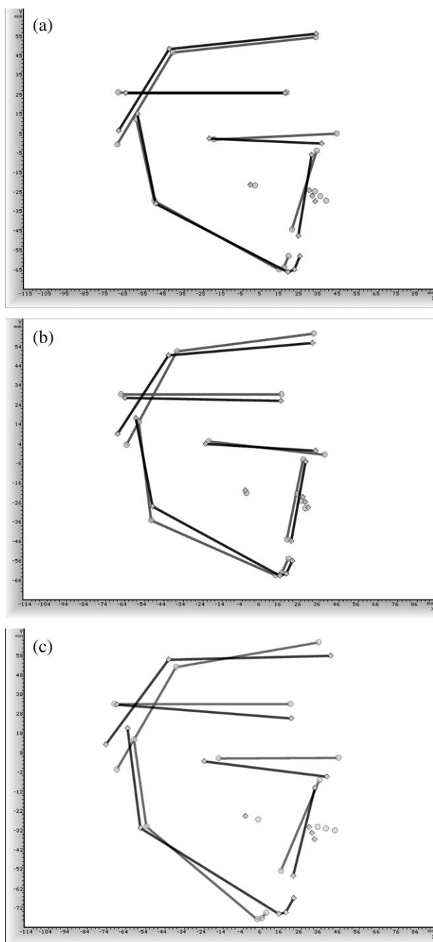
Figure 8 Examples of the morphometric application of the currently proposed technique to various patients. The template is depicted in black (squares) and the patient in grey (circles). In (a), the superimposition seems to suggest a short, retrognathic mandible, combined with slight maxillary prognathism, and a favourable mandibular plane angle. For the patient in (b), the maxillomandibular relationship seems to be normal, albeit with slight bimaxillary retrusion, a minor retrusion of the chin due to a somewhat shorter mandibular corpus, and an increased lower posterior face height. In (c), the proposed technique is applied to a surgery patient. A marked mandibular retrusion is combined with a minor maxillary protrusion and a considerably increased lower anterior face height. The dentition is clearly protrusive. Interestingly, the superimposition indicates posterior maxillary intrusion and mandibular autorotation/slight protrusion using a bimaxillary surgical approach as the treatment regimen for this patient.
